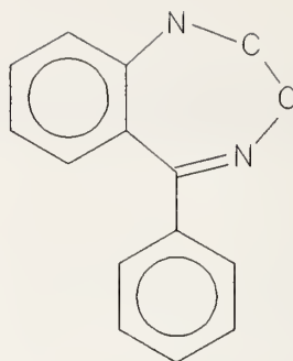
FIGURE 1 1,4-Benzodiazepine Structure
